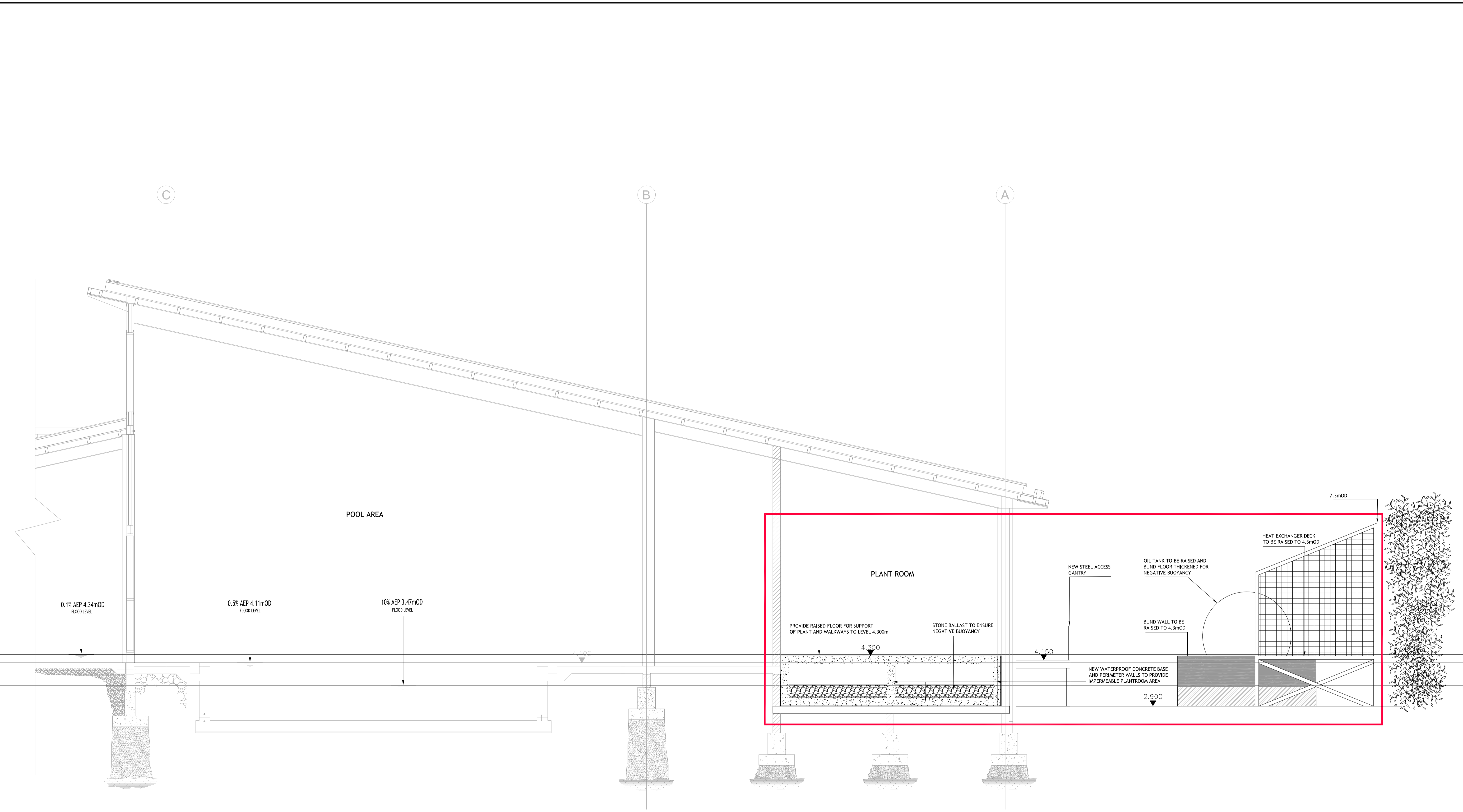
PROPOSED CROSS SECTION 111-01 1:50 A1 1:100 A3
