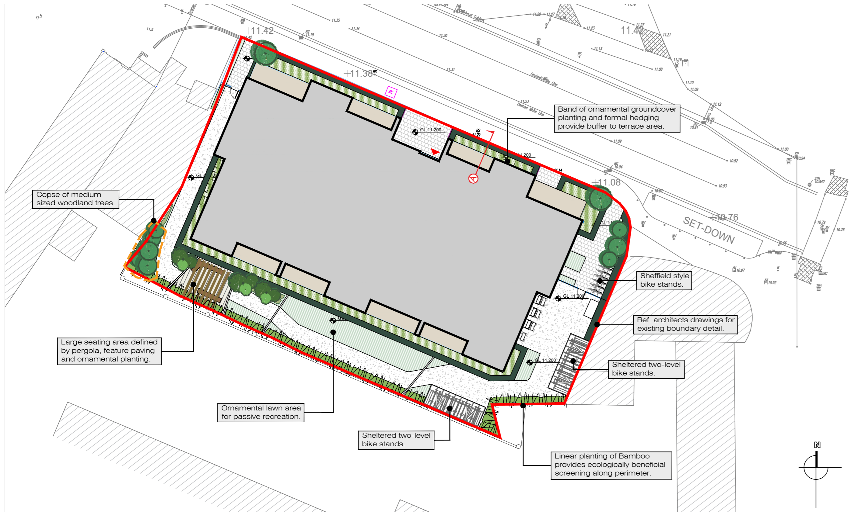
Landscape Masterplan | 1: 250
