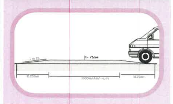
Diagram 6.34 Cross section of 75mm high flat-top ramp
