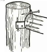
DETAIL 6 - GALVANISED STEEL BRACE PLATE (FIXING DETAIL)
