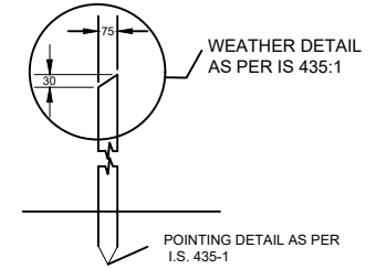
SECTION 1 POINTING DETAIL
