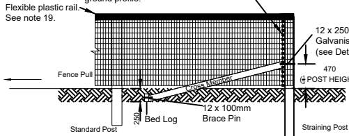
DETAIL 2 - END POST ASSEMBLY ELEVATION
