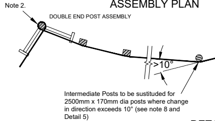
Detail 3 - END POST ASSEMBLY PLAN
