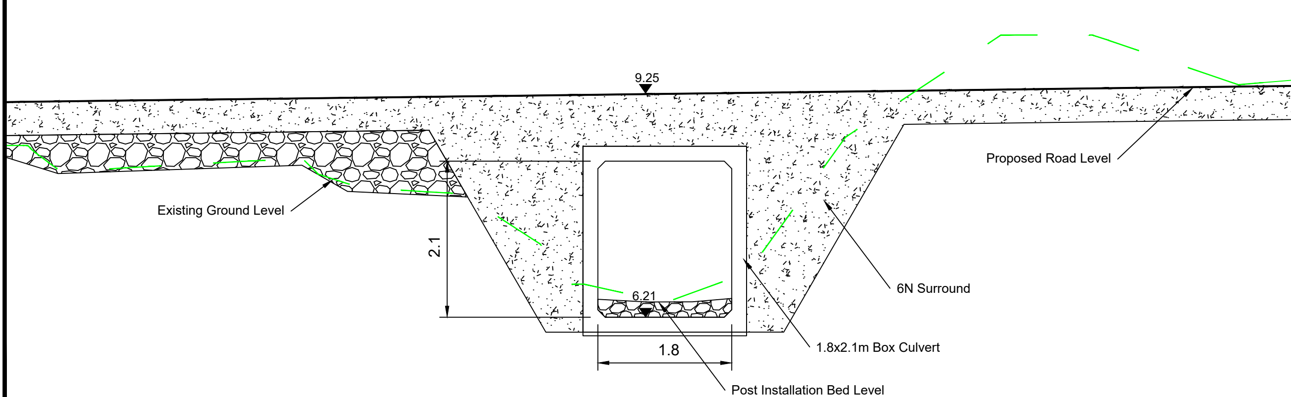
Section C-C
