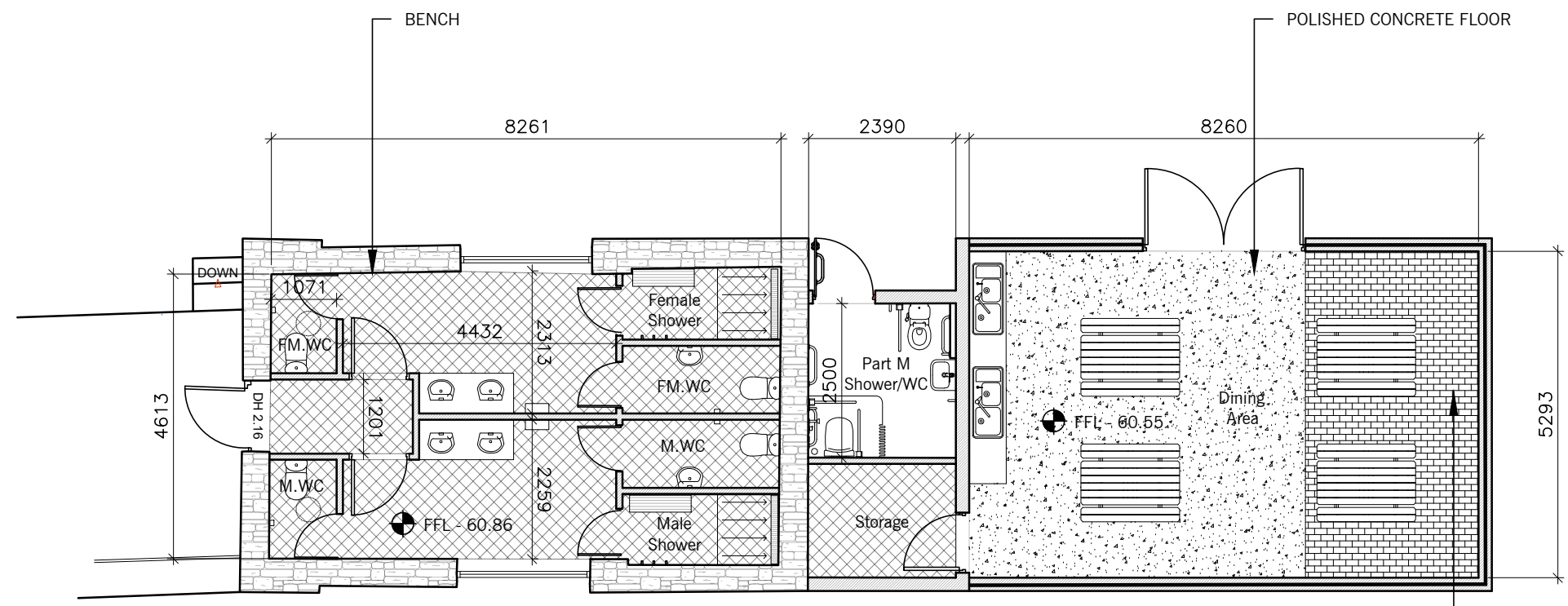
01 203 GROUND FLOOR PLAN SCALE 1:100
