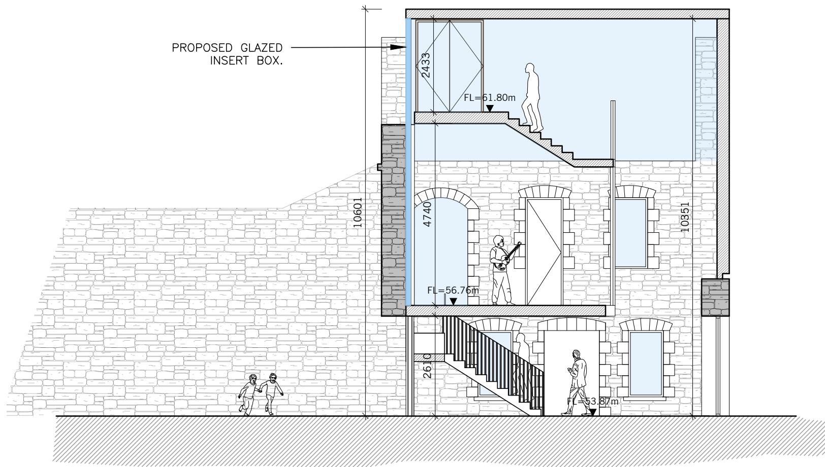
01 209 PROPOSED SECTION BB SCALE 1:100
