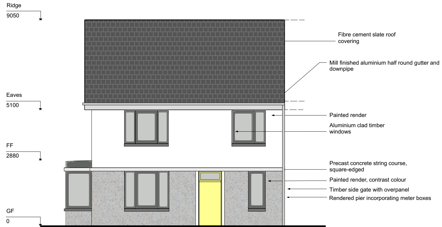
4B-7P Terrace Appendage Elevation A
