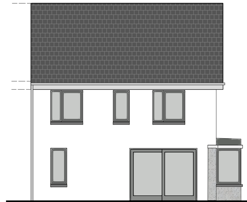
4B-7P Terrace Appendage Elevation B
