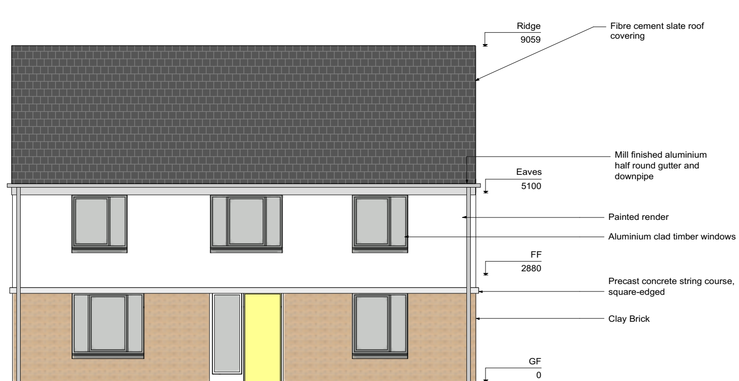
4B + 1 Community Houses Elevation A
