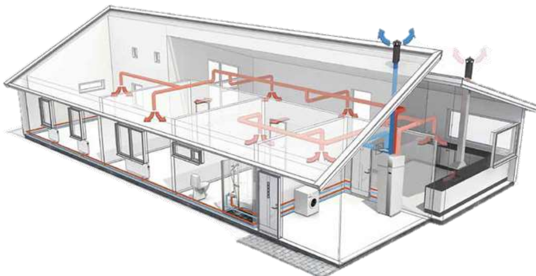
Figure 9: Exhaust Air Heat Pump System
