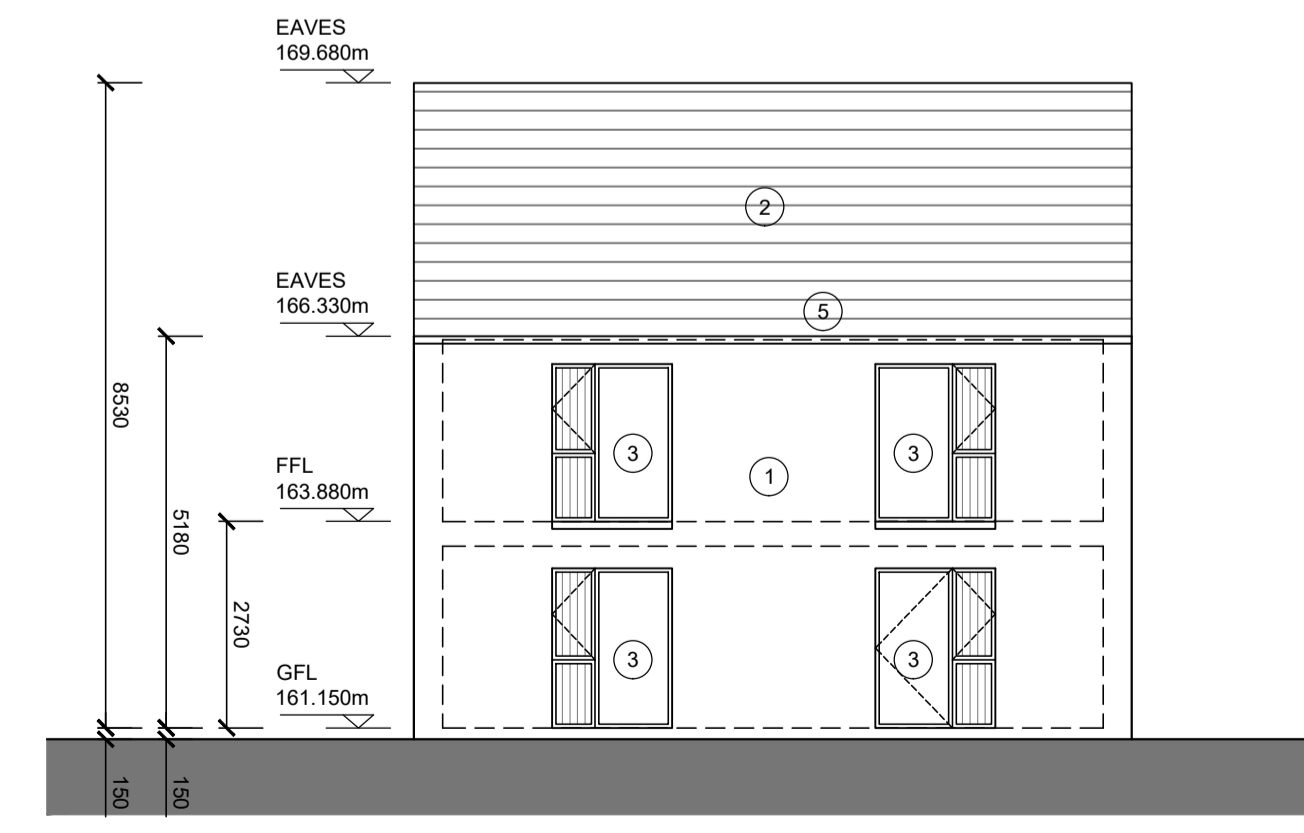
HOUSE No. 10 (TYPE A1) ELEVATION 4
