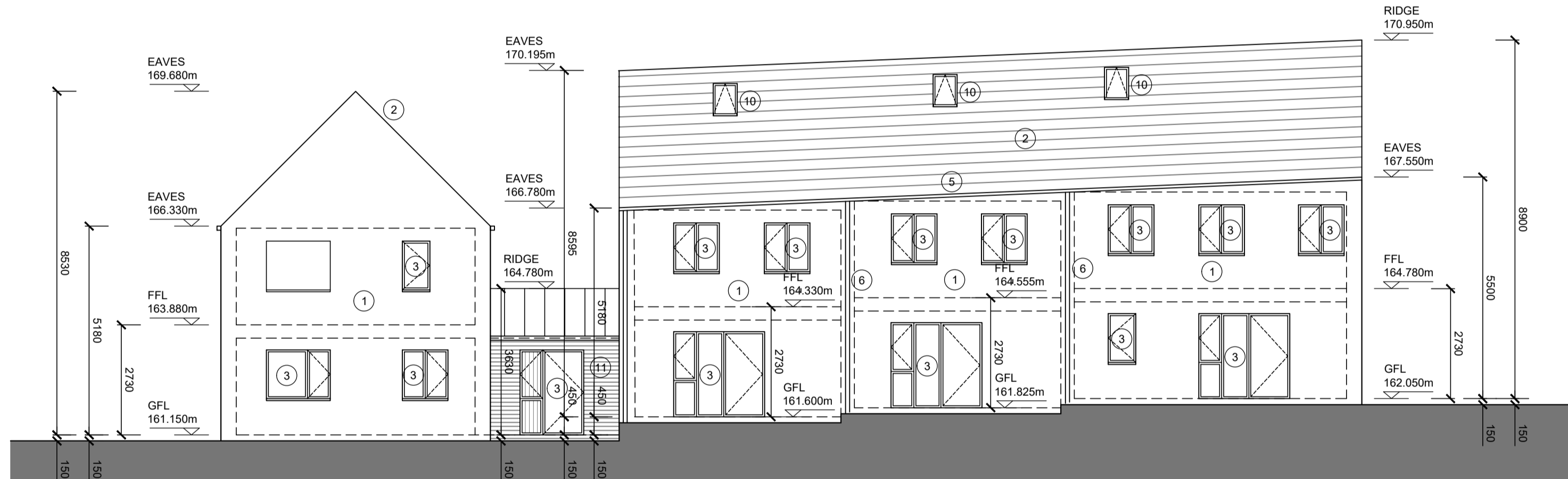
HOUSE No. 10 (TYPE A1) HOUSE No. 9 (TYPE C) HOUSE No. 8 (TYPE C) HOUSE No. 6 (TYPE D2) ELEVATION 2
