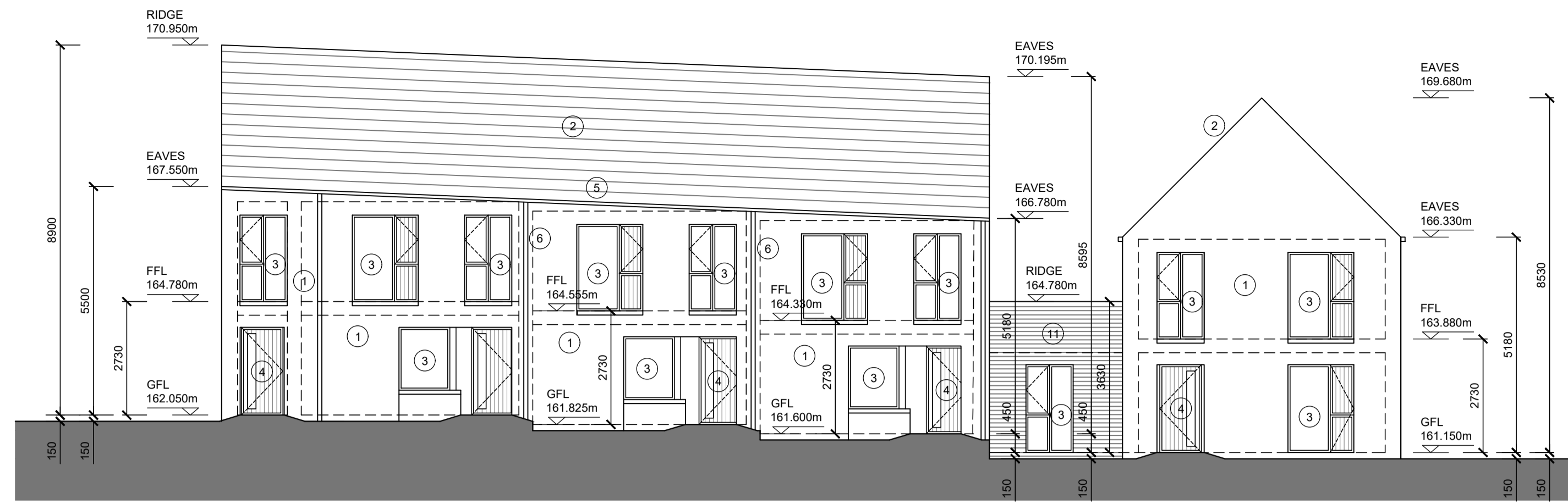
HOUSE No. 6 (TYPE D2) @ FFL HOUSE No. 7 (TYPE D1) @ GFL HOUSE No. 8 (TYPE C) HOUSE No. 9 (TYPE C) HOUSE No. 10 (TYPE A1) ELEVATION 1
