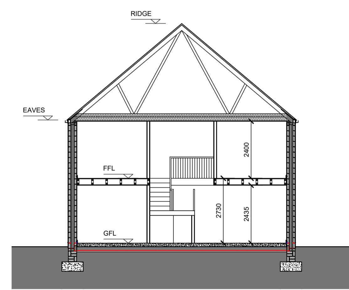
CROSS SECTION A-A
