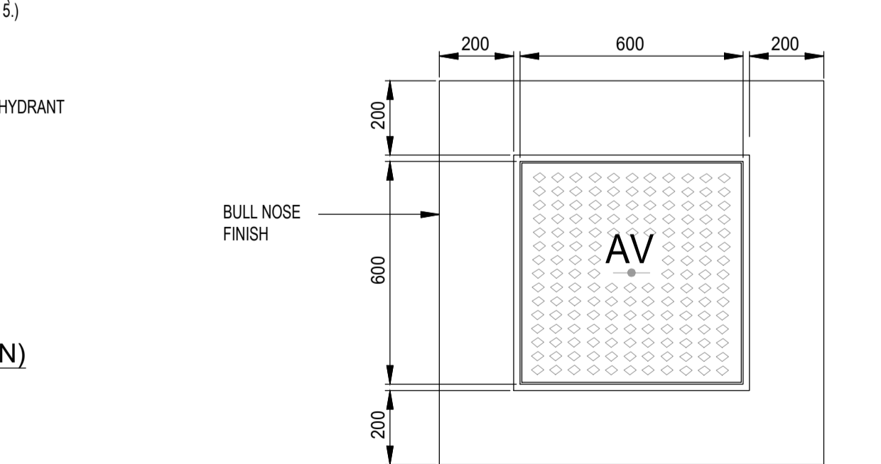
IRISH WATER DETAIL STD-W-22 ON LINE AIR VALVE FOR POLYETHYLENE (P.E.) PIPE SCALE: NTS
