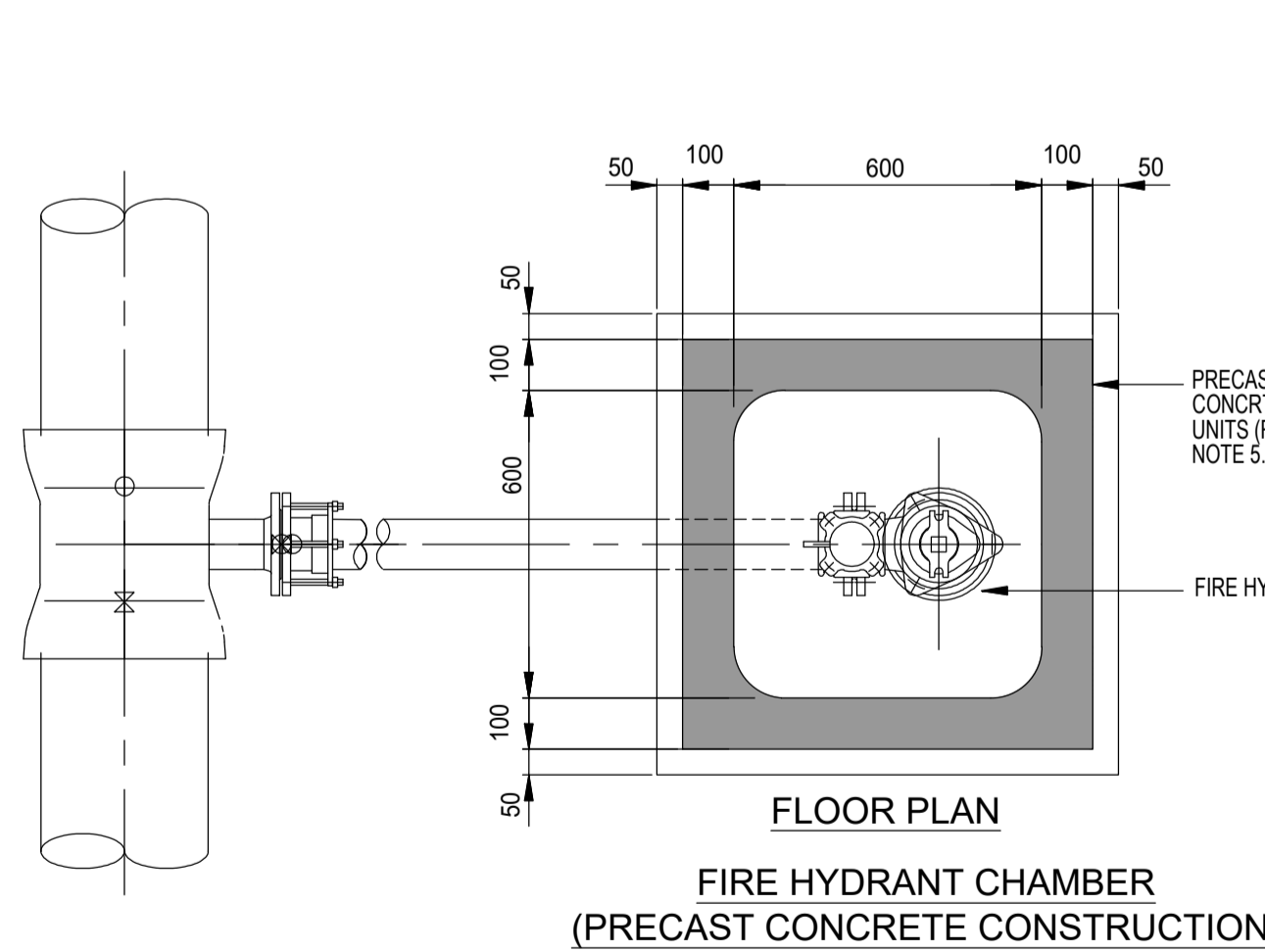
IRISH WATER DETAIL STD-W-19 OFF LINE HYDRANT FOR POLYETHYLENE (P.E.) PIPE SCALE: NTS
