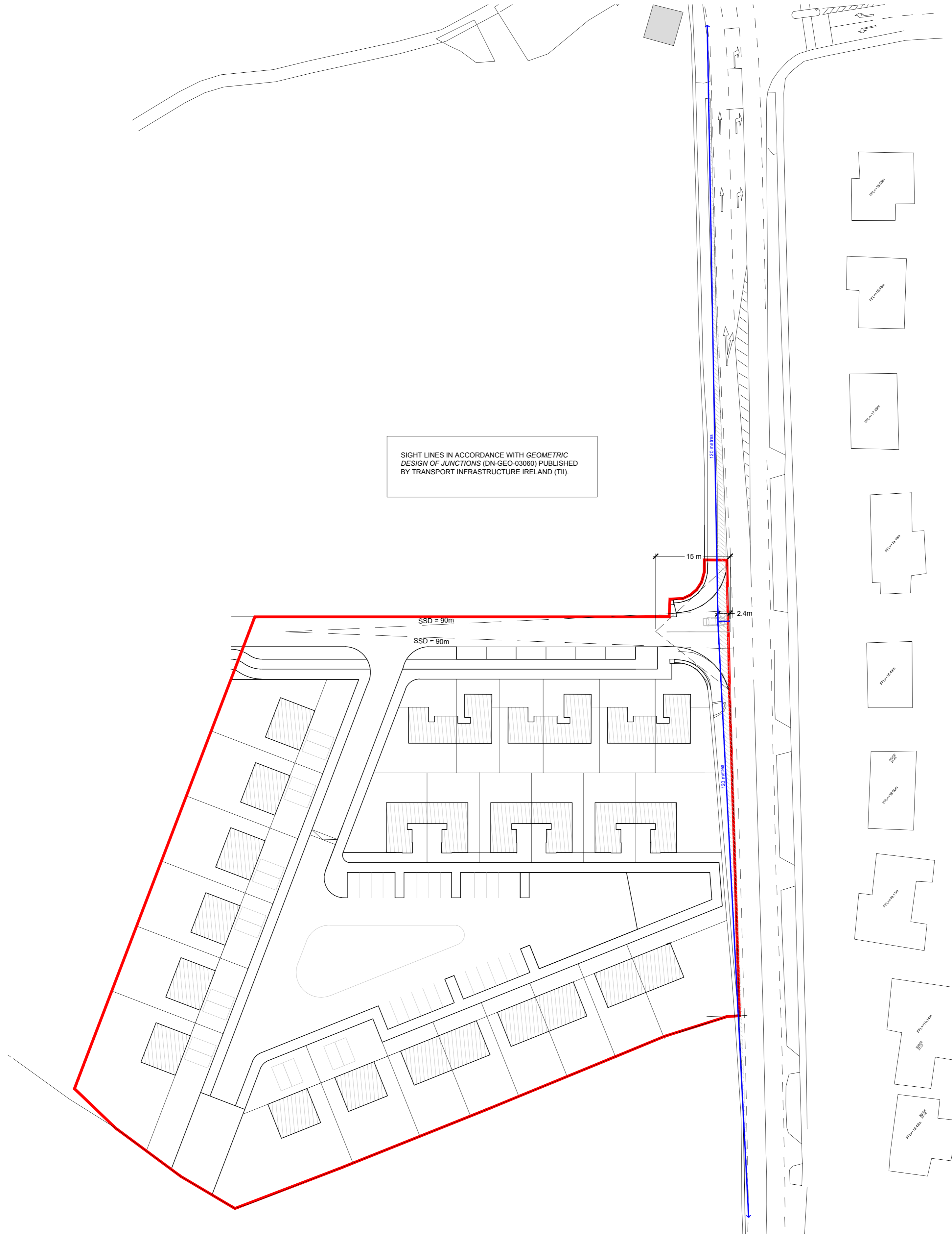
SIGHTLINE COMPLIANCE- PLAN SCALE 1:500@ A1
