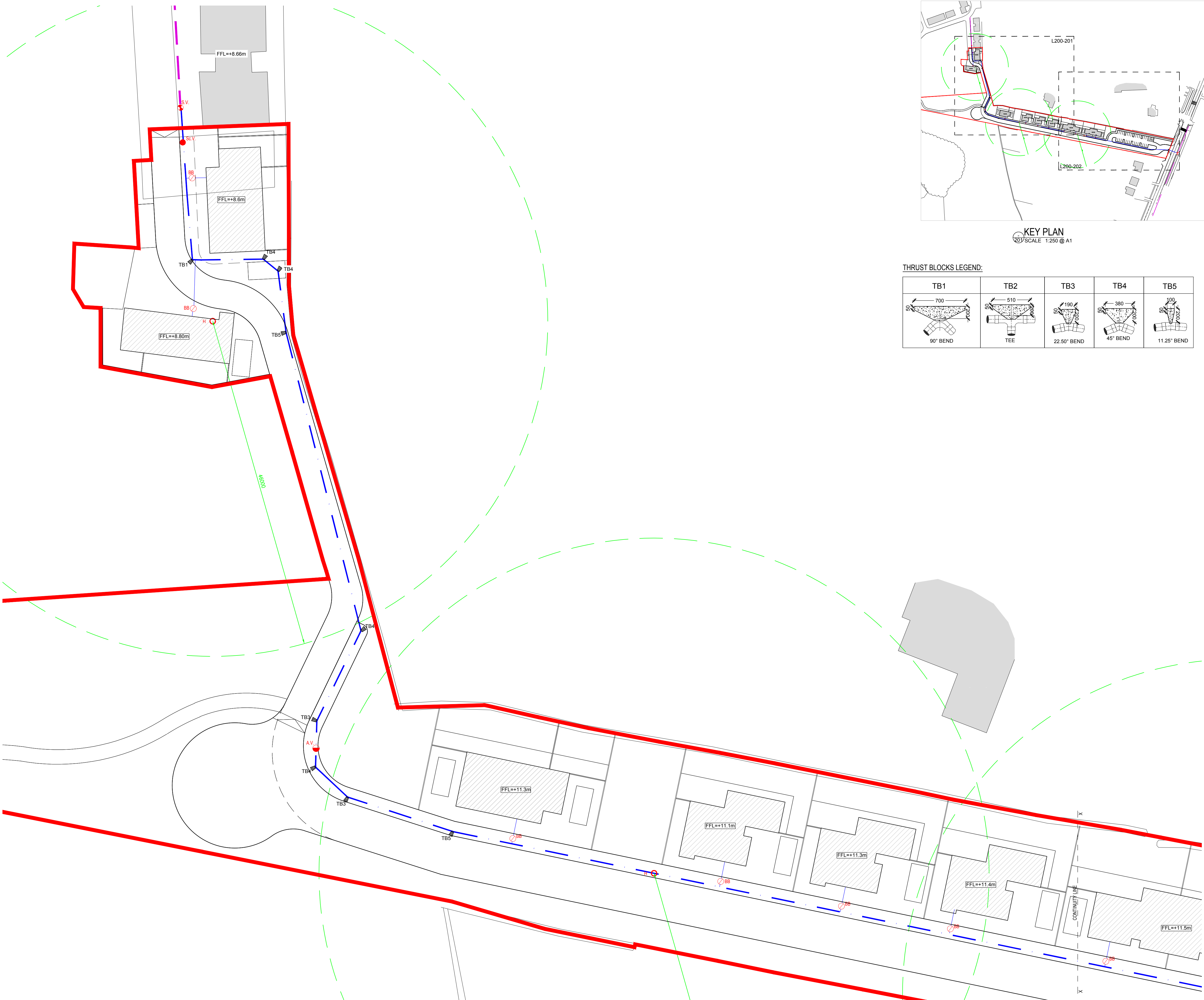
PROPOSED WATER MAIN LAYOUT- DWG 1 OF 2 SCALE 1:250 @ A1
