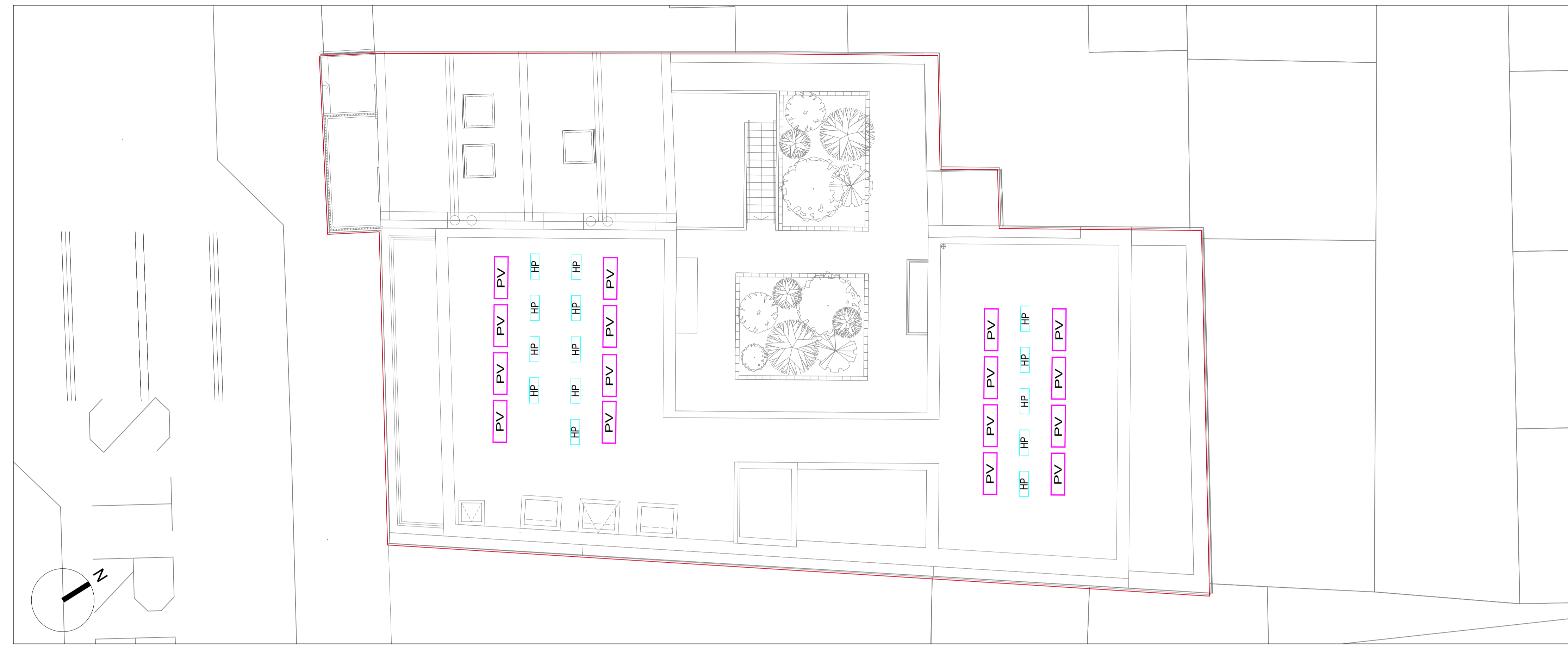
PV PANEL & HEAT PUMP ROOF LAYOUT SCALE 1:100
