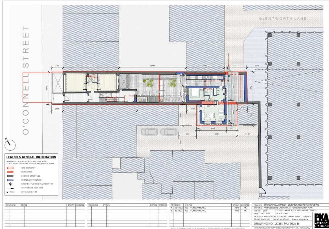
Figure 3 – Site layout (ground floor)
