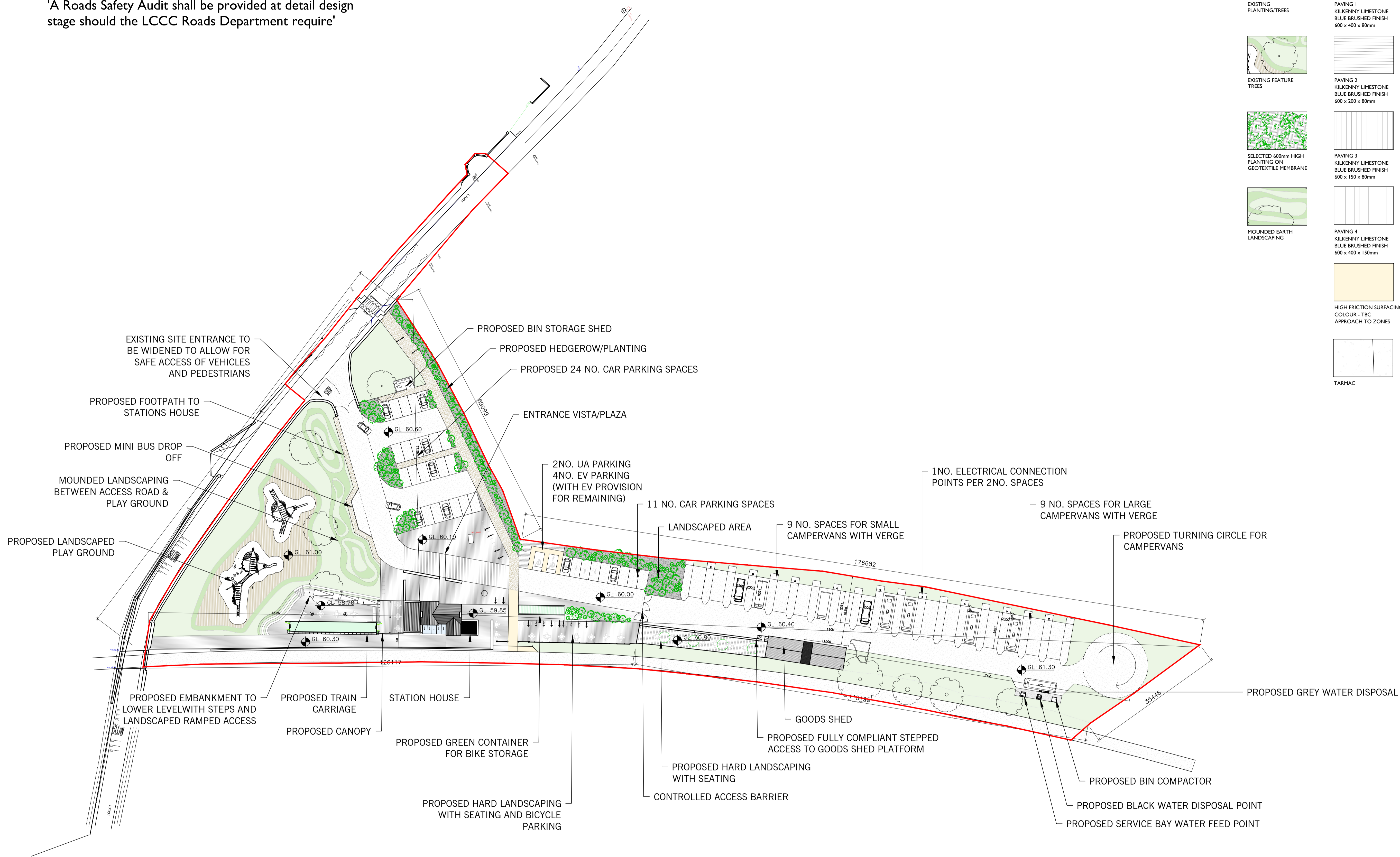
01 202 PROPOSED SITE LAYOUT PLAN SCALE 1:500
