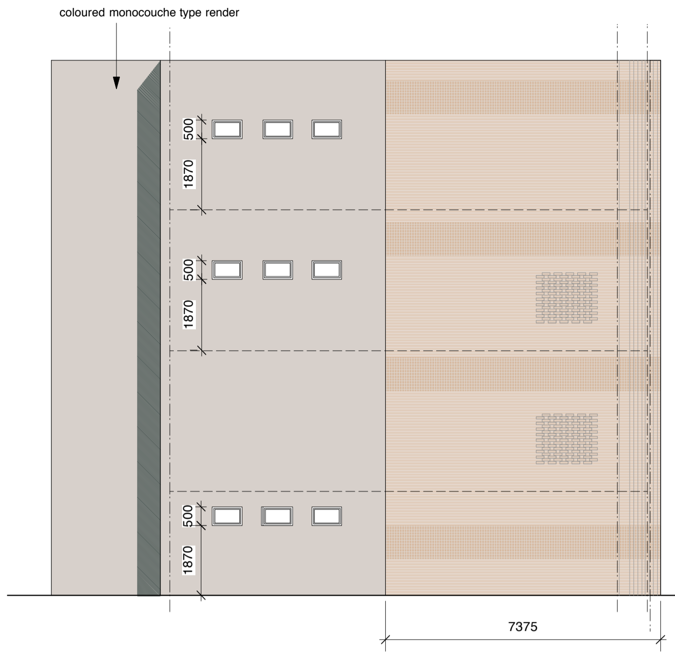
Lane/ Gable Elevation
