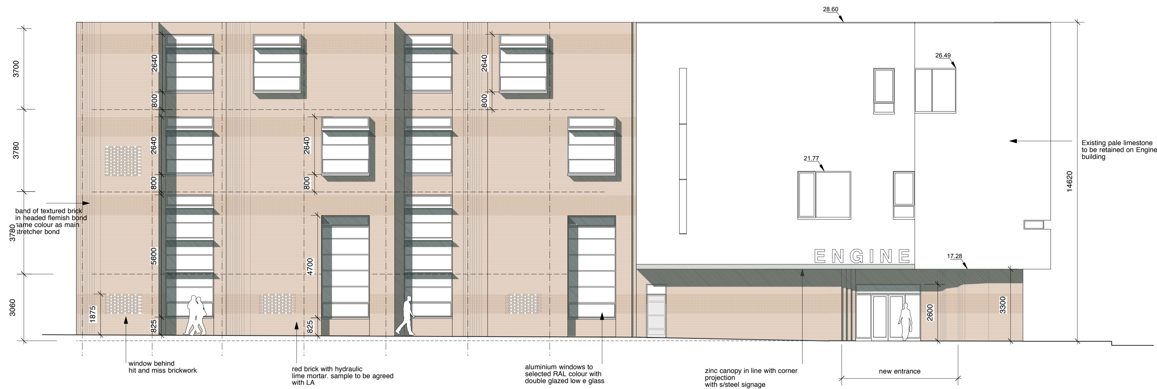
Dominic Street Elevation
